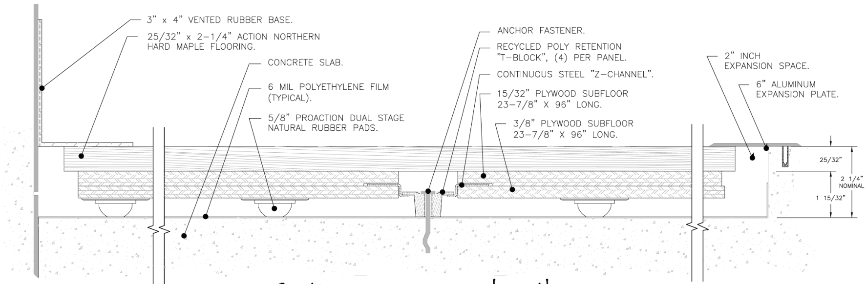
Section across room length
