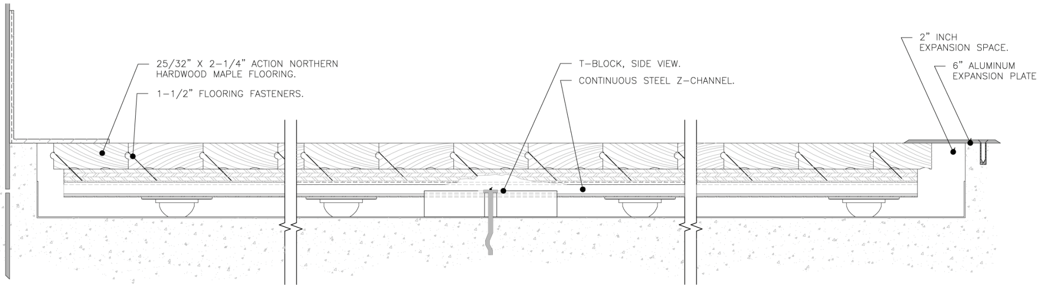
Section across room width
