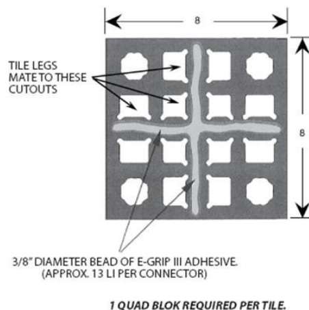
2. Connector Detail
